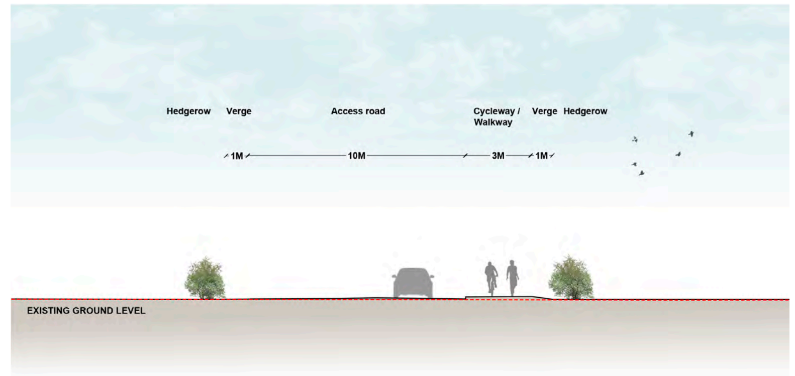
Section O-O'
