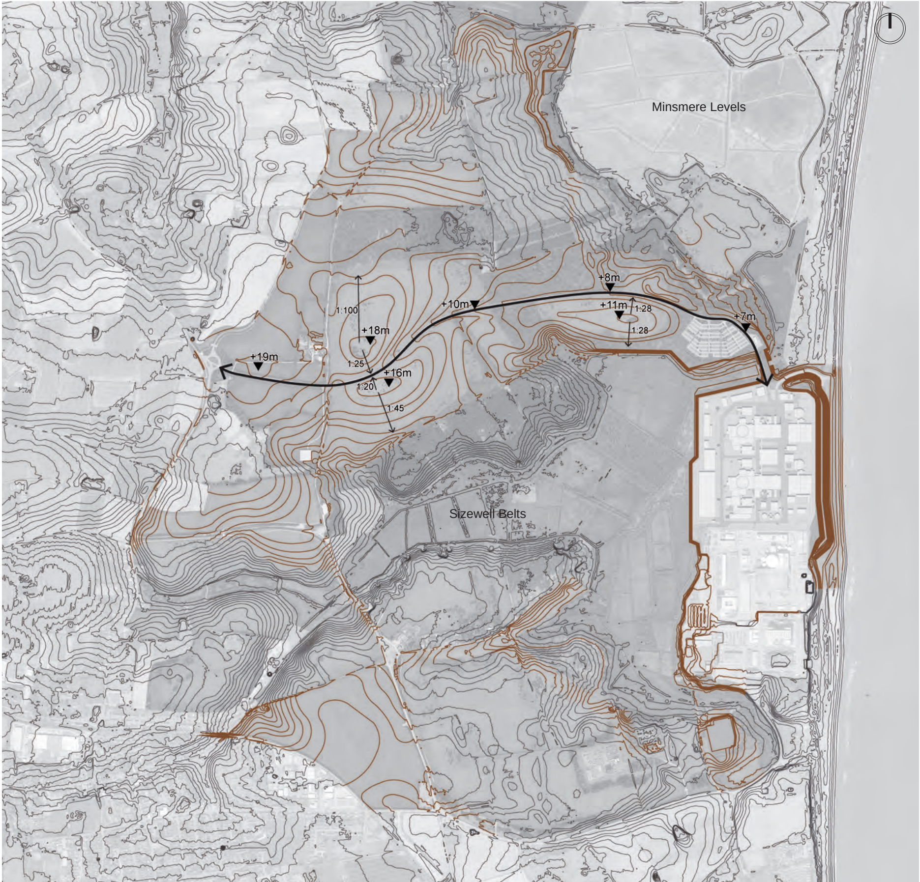
Figure 8.15: Indicative landform strategy (SZB relocated facilities Option 2 layout)
