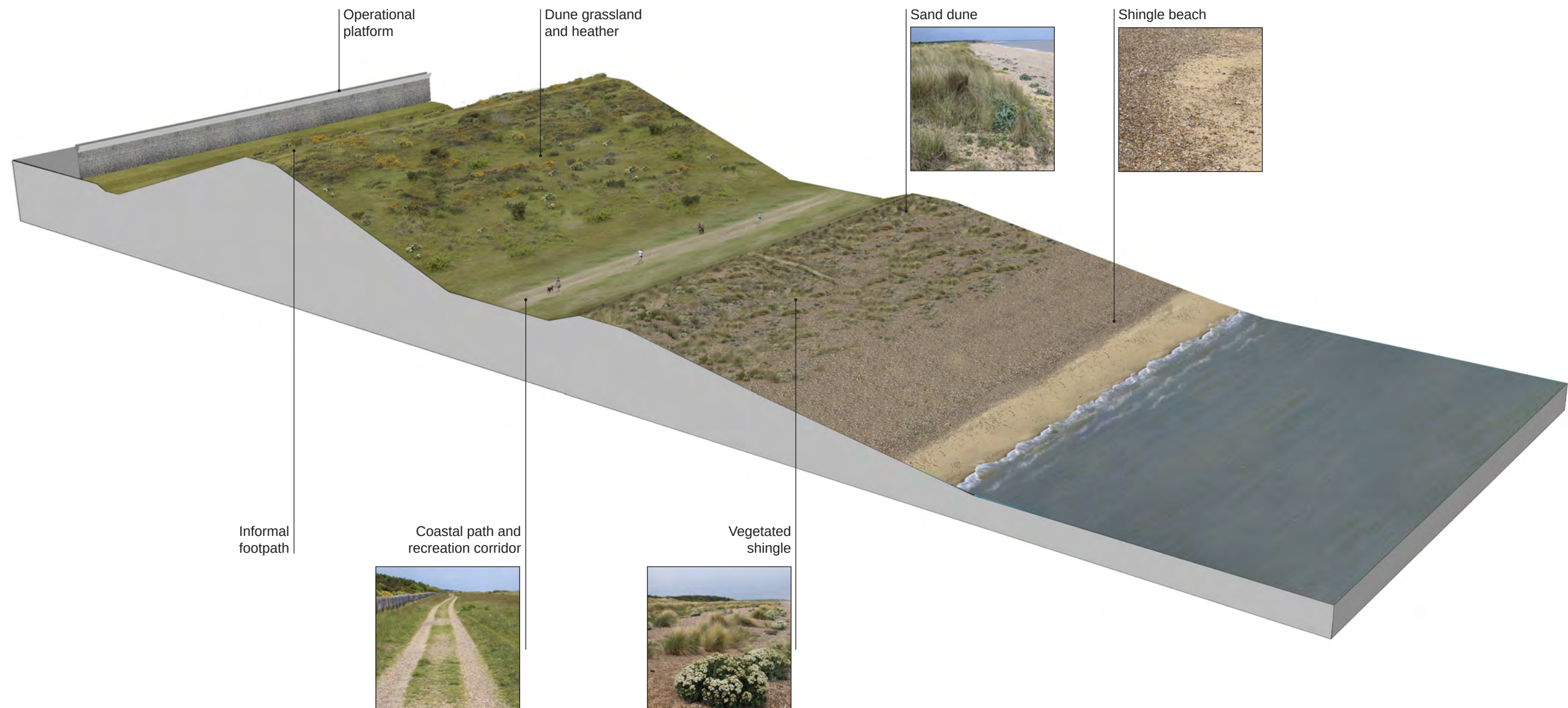
Figure 8.27: Visualisation of the sea defence
