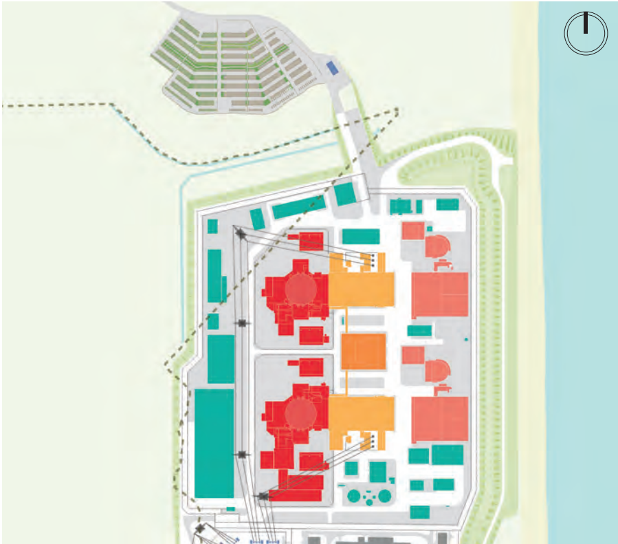
Figure 7.68: Sizewell C overview
