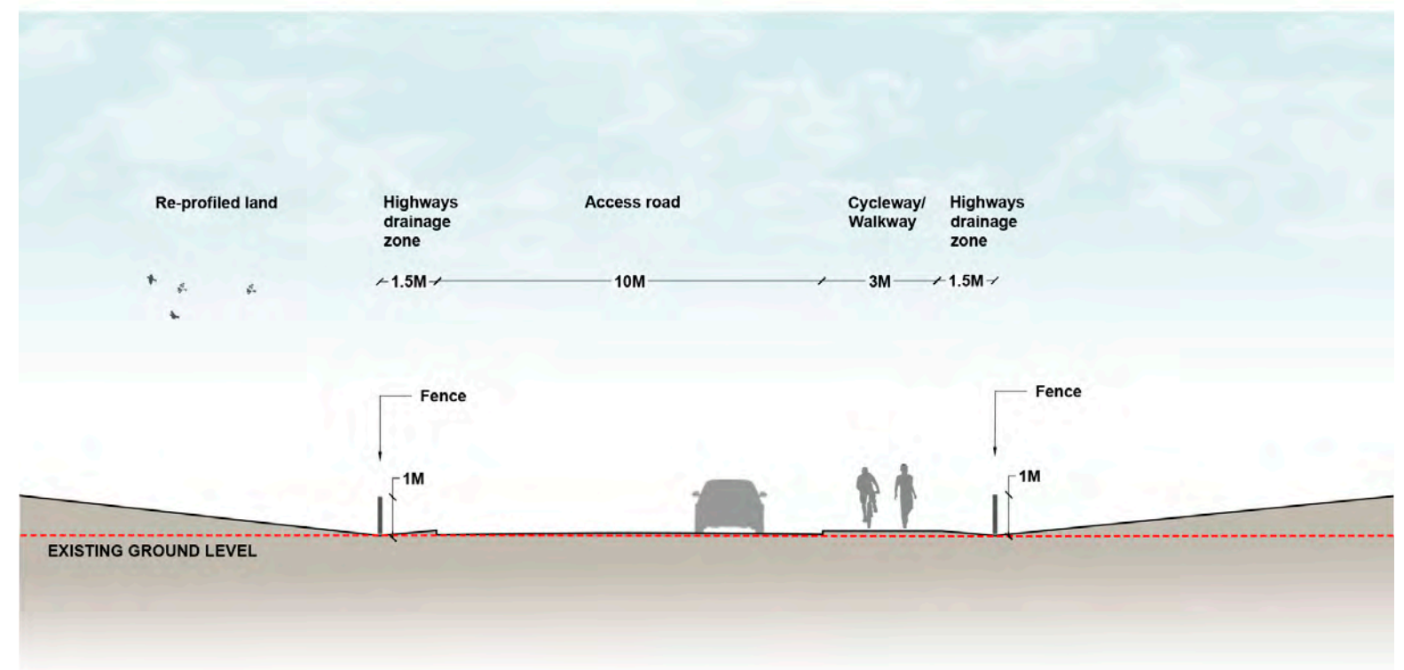
Section P-P'
