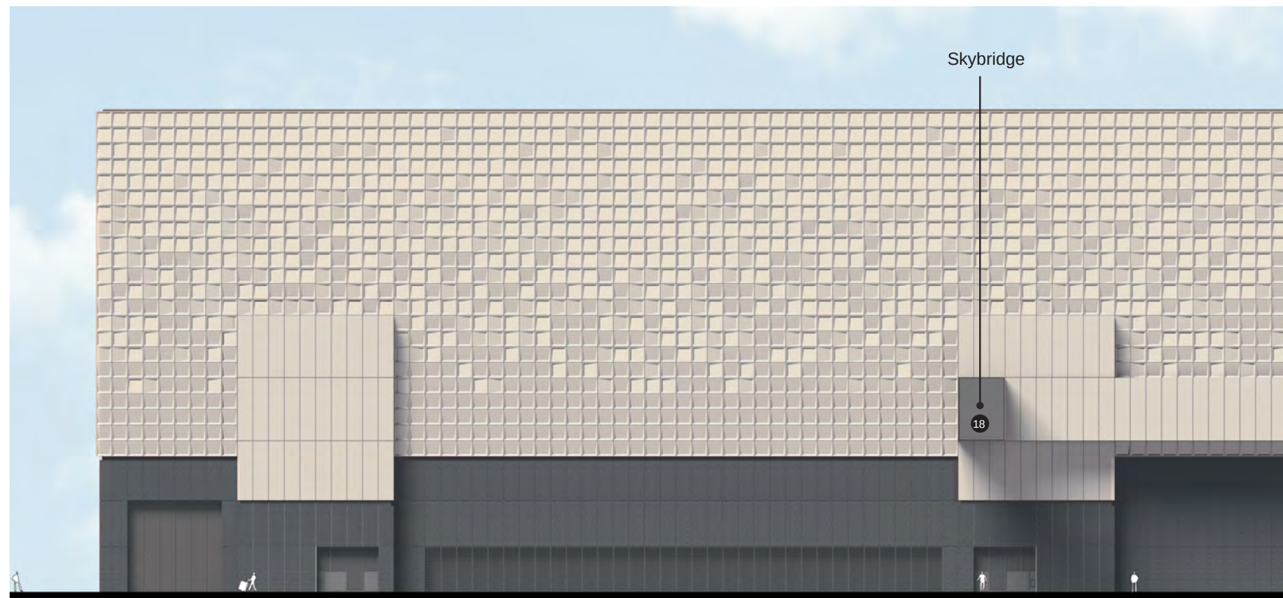
Figure 7.42: Turbine hall unit 1 north elevation, at 1:500
