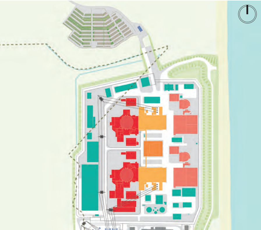
Figure 7.48: Sizewell C overview
